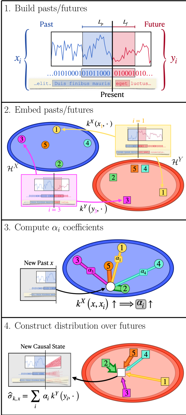
FIG. 2. The empirical kernel causal state algorithm. Step 1: Build a library of past sequences x_i and future sequences y_i from observed data. Step 2: Construct an appropriate kernel for pasts k^X and a kernel for futures k^Y . Embed pasts (circles) and futures (squares) into their respective Hilbert spaces, \mathcal{H}^X (blue) and \mathcal{H}^Y (red). Step 3: Calculate the empirical kernel causal state embedding coefficients \alpha_i for a new past x by comparing x to each embedded past x_i . More similar pasts will have larger embedding coefficients. Step 4: Construct the distribution over futures for x using the calculated \alpha_i to weight the sum over the associated futures y_i .
