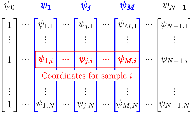
FIG. 3. Relation between the causal diffusion components \psi —the eigenvectors of the diffusion matrix M^{S_k} —and the coordinates that encode the empirical kernel causal states.
