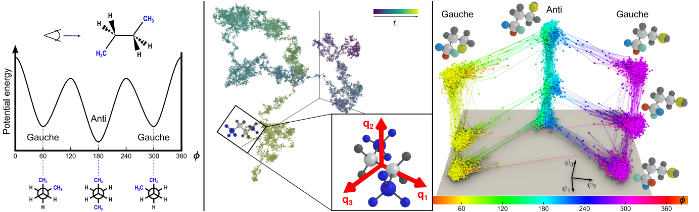
FIG. 7. Left: The potential energy of n -butane molecule plotted along the dihedral angle \phi . The Newman projection for each of the three low energy conformations is shown below the plot. Middle: The global trajectory of the simulated n -butane molecule under Brownian motion. The inset shows the local frame of the molecule position used as input to the empirical kernel causal state algorithm. Only the carbon in the back is mobile in this local frame. Right: The empirical kernel causal state set of the n -butane molecule, embedded using the first three causal diffusion components. The frame shows the base vectors in \mathbb{R}^3 , scaled down to fit in the figure. These give the directions along which the values \psi_{j,i} are plotted, for j = 1, 2, 3 indicated on the figure and i each data index. Dots are plotted at the locations of each \hat{\sigma}_{x_i} and lines connect successive samples in time. Nine clusters are clearly apparent. The average position of each atom in a selection of these clusters is shown, with the free carbon (yellow) and hydrogens of the fixed methyl group (red, green, and blue) highlighted.
