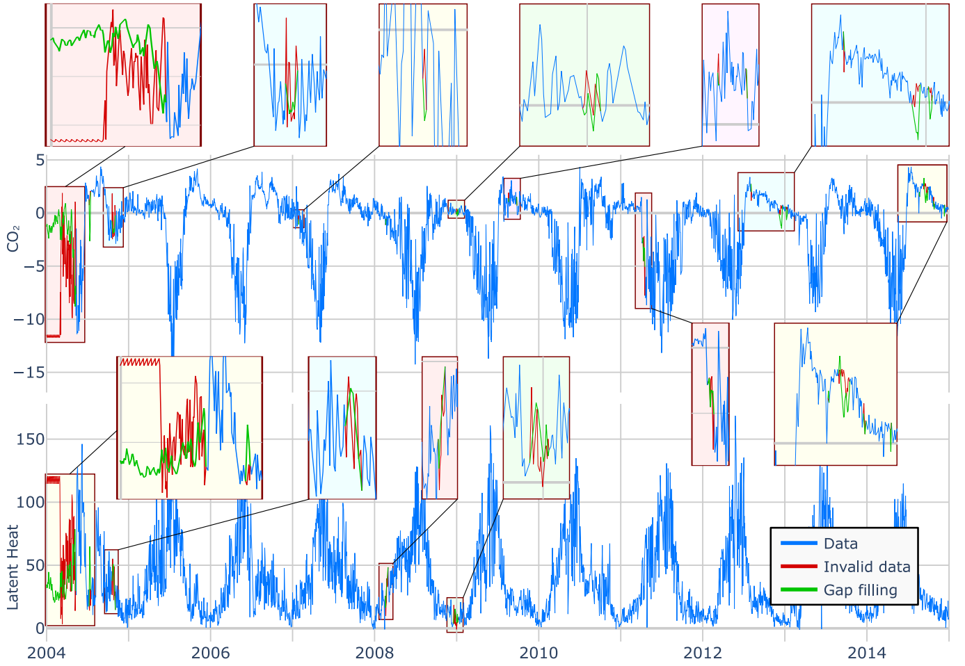
FIG. 11. \text{CO}_2 and Latent Heat flux data from the crop example in Section V B. Data in red is marked as invalid and should not be seen as a target for the gap-filled data (in green). This is especially apparent for the first few months of 2004. Data in blue could also be of low quality, especially at each gap boundary. The gap-filled sections look plausible and are consistent with the measurements of all other variables.
