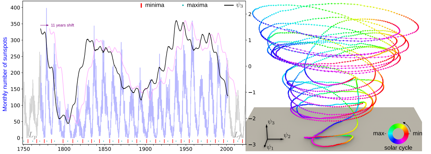
FIG. 9. Left: Monthly number of sunspots since 1749. Dates of solar minima and maxima are indicated below the main plot. The third diffusion component is overlaid on the data in black. Shifting this component by eleven years, maximizing the correlation of the sunspots data and \psi_3 , clarifies that \psi_3 approximately predicts the amplitude of the next solar cycle. Right: The empirical kernel causal states of the sunspot sequence, embedded using the first causal diffusion components. The indicated frame, dots and lines in the figure have the same interpretation as in Fig. 7. The color map indicates the solar cycle phase at the time t associated with each \hat{\sigma}_{x_t} . This phase was computed by linearly interpolating the time between each solar minima and maxima.
