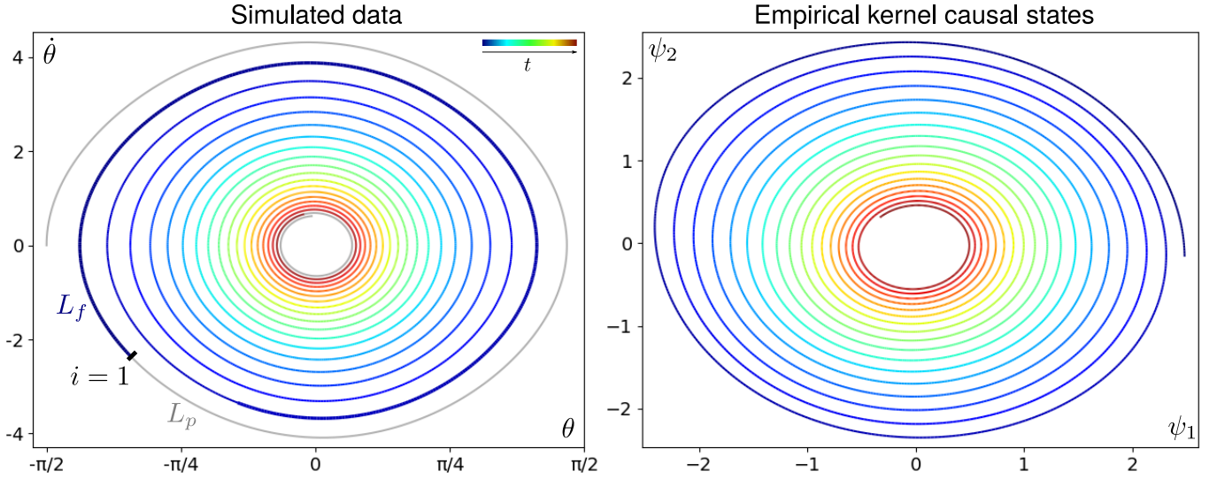
FIG. 6. Left: The pendulum trajectories in the angle and angular velocity (\theta, \dot{\theta}) parameter plane colored by time. The gray sections at the beginning and end are the first L_p -length past and last L_f -length future, respectively, and so do not correspond to any embedded causal states. The bold segment denotes the L_f -length future for the first embedded history. Right: The empirical kernel causal states plotted using their first two diffusion coordinates.
